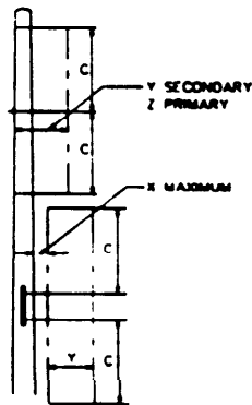
VERTICAL DIMENSIONS OF CLIMBING SPACE COLUMN
