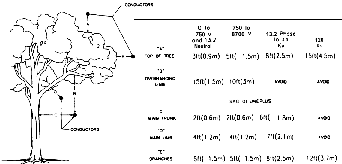
Figure 4-24. Recommended minimum clearances for tree trimming
