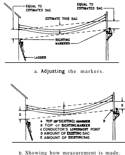
Figure 4-11. Measuring sag on service drop conductors
