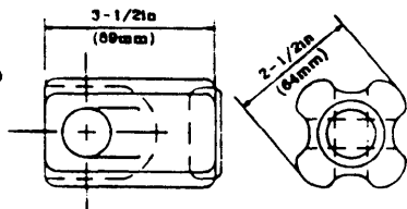
GUY STRAIN, CLASS 54-1
